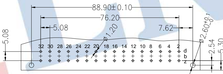
Recommended P.C.B Layout(Top Side) (PCB BOARD TOLERANCE±0.05)
