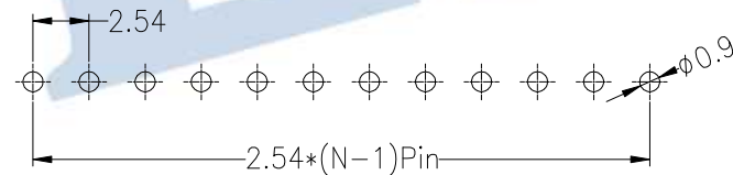
Recommended P.C.B Layout(Top Side) (PCB BOARD TOLERANCE±0.05)
